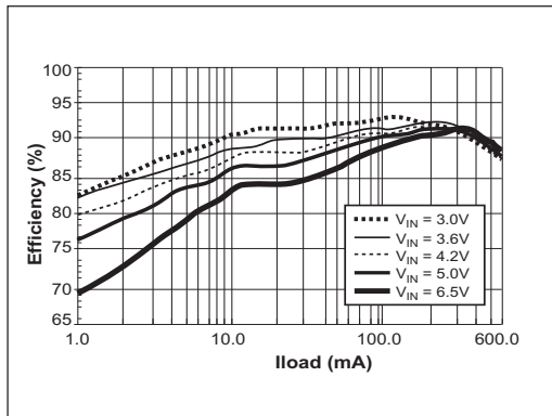
Figure 4. Efficiency vs. Output Current, V_{OUT} = 2.5V , L1 = 22\mu H (Sumida CDRH6D28), I_{LIM} = V_{IN}
