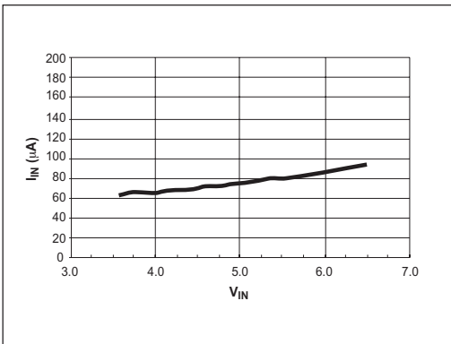
Figure 3. No Load Battery Current, V_{OUT} = 3.3V , L1 = 22\mu H (Sumida CDRH6D28), I_{LIM} = V_{IN}
