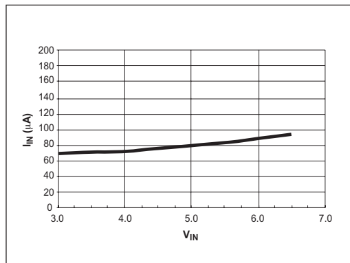
Figure 6. No Load Battery Current, V_{OUT} = 2.5V , L1 = 22\mu H (Sumida CDRH6D28), I_{LIM} = V_{IN}
