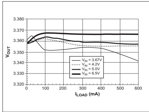
Figure 2. Line/Load Rejection, V_{OUT} = 3.3V , L1 = 22\mu H (Sumida CDRH6D28), I_{LIM} = V_{IN}
