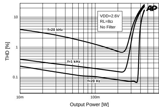
Figure 6. THD+N vs. Output Power, VDD =2.6V
