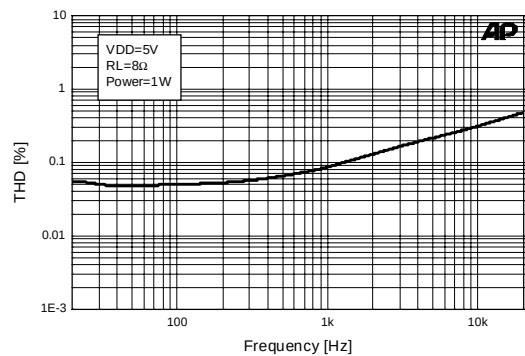
Figure 1. THD+N vs. Frequency, VDD =5V
