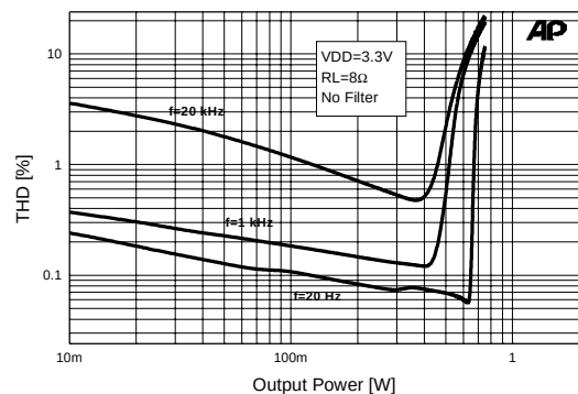
Figure 5. THD+N vs. Output Power, VDD =3.3V
