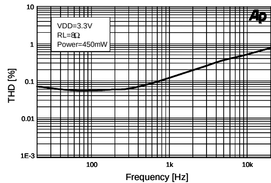
Figure 2. THD+N vs. Frequency, VDD =3.3V
