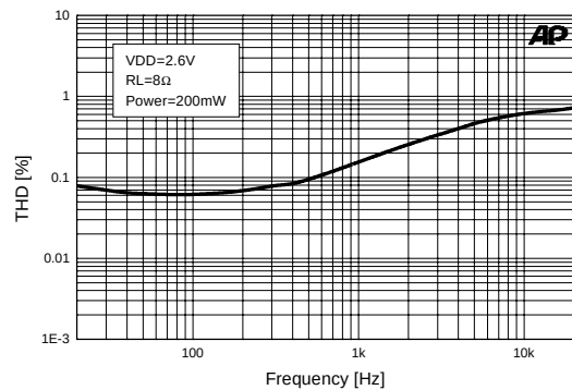
Figure 3. THD+N vs. Frequency, VDD =2.6V
