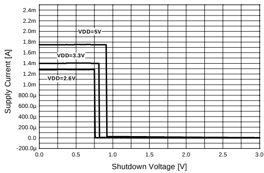
Figure 15. Supply Current vs. Shutdown Voltage
