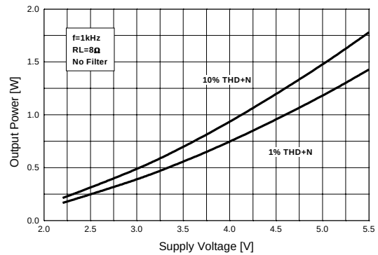
Figure 16. Output Power vs. Supply Voltage
