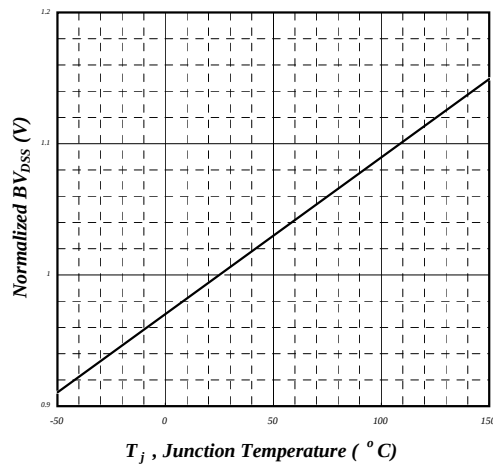
Fig 3. Normalized BV_{DS} v.s. Junction Temperature
