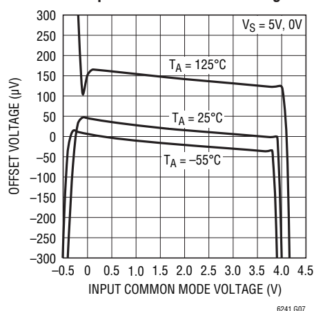
Offset Voltage vs Input Common Mode Voltage
