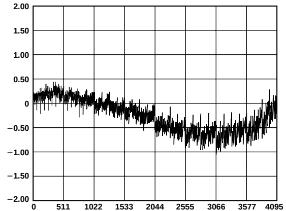
Figure 5. Typical INL
