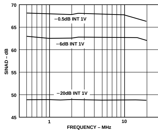
Figure 6. SINAD vs. Input Frequency (Input Span = 2 V p-p, V_{CM} = 2.5 V Differential Input)
