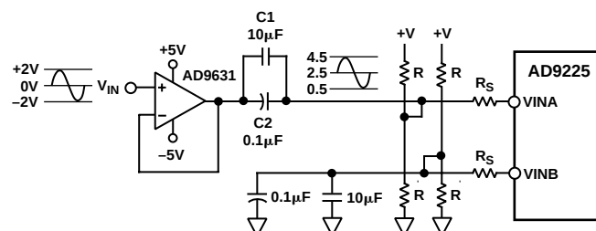
Figure 21. AC-Coupled Input
