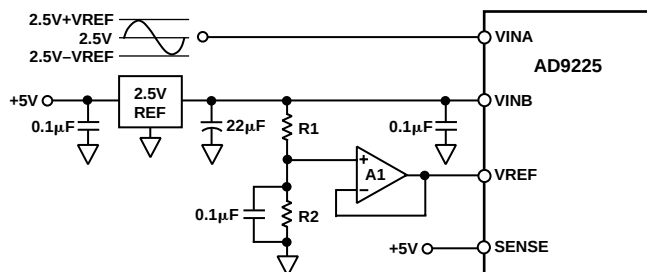
Figure 29. External Reference
