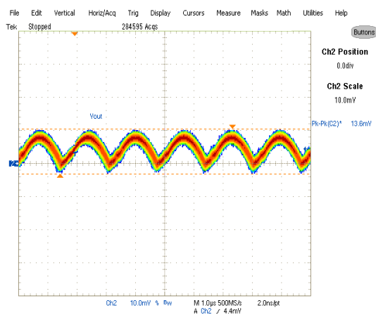
Fig. 20: Output Voltage Ripple, 8A load Ch 2 : V_{out}
