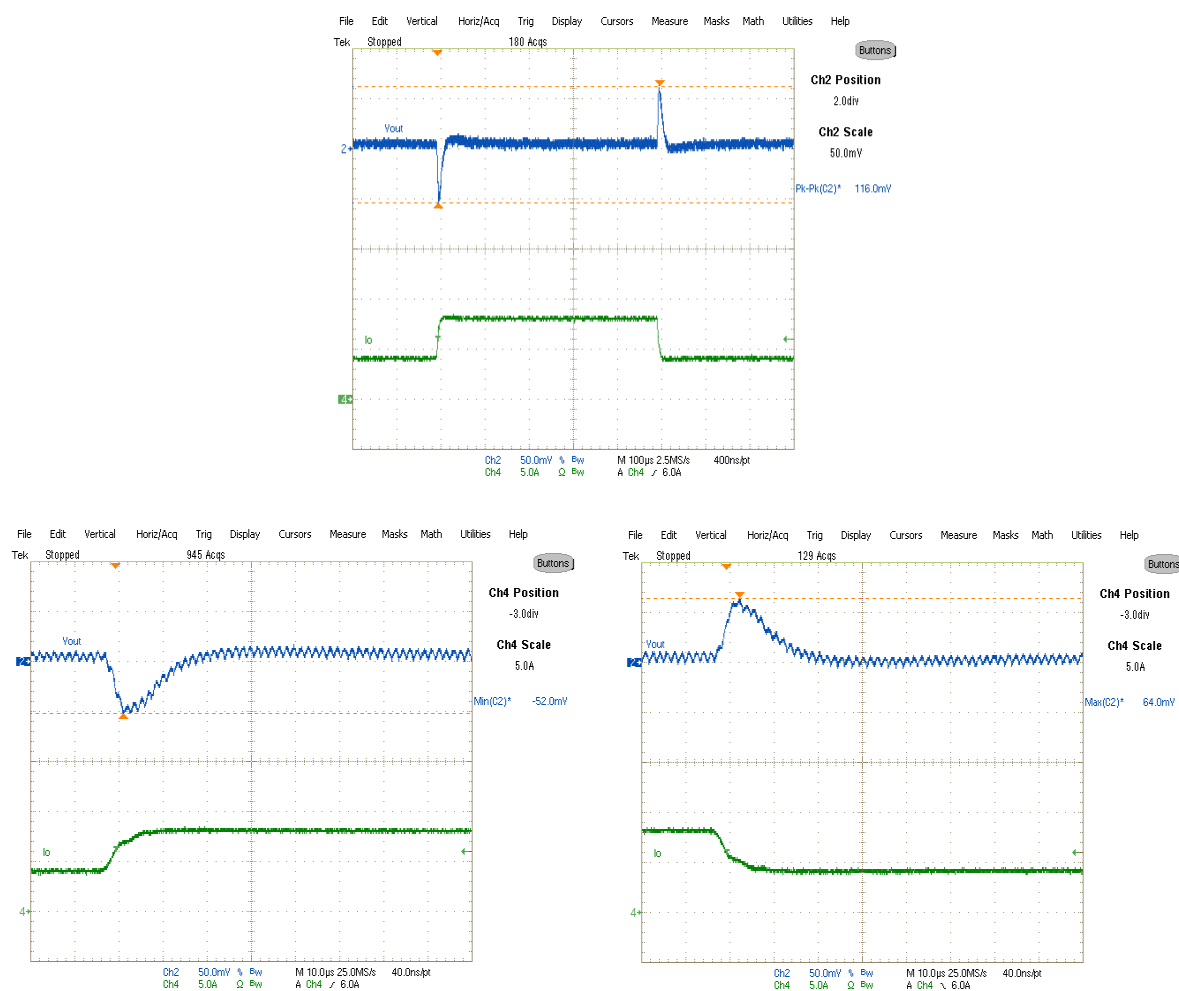
Fig. 23: Transient Response, 4A to 8A step 2.5A/us Ch 2 :V out , Ch 4 :I out
