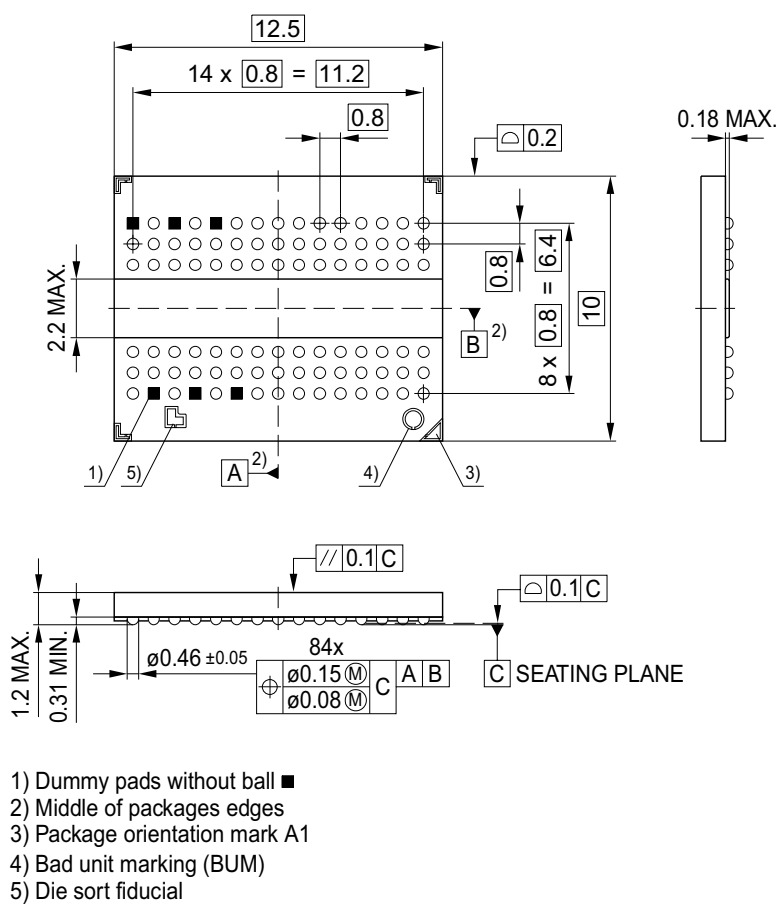
FIGURE 9 Package Outline PG-TFBGA-84
