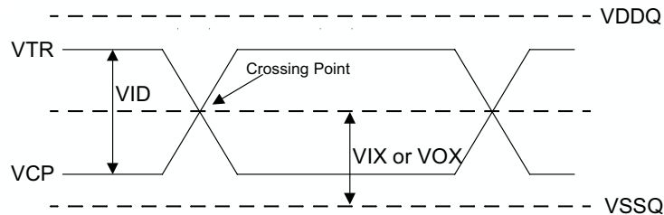
FIGURE 3 Differential DC and AC Input and Output Logic Levels Diagram
