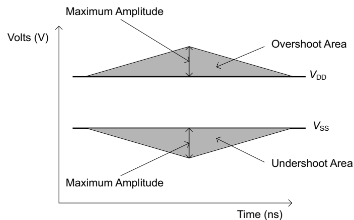
FIGURE 4 AC Overshoot / Undershoot Diagram for Address and Control Pins
