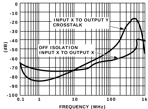
FIGURE 9. EL4340 CROSSTALK AND OFF-ISOLATION
