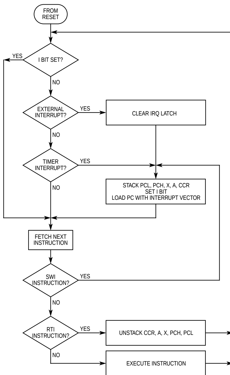
Figure 4-4. Interrupt Flowchart
