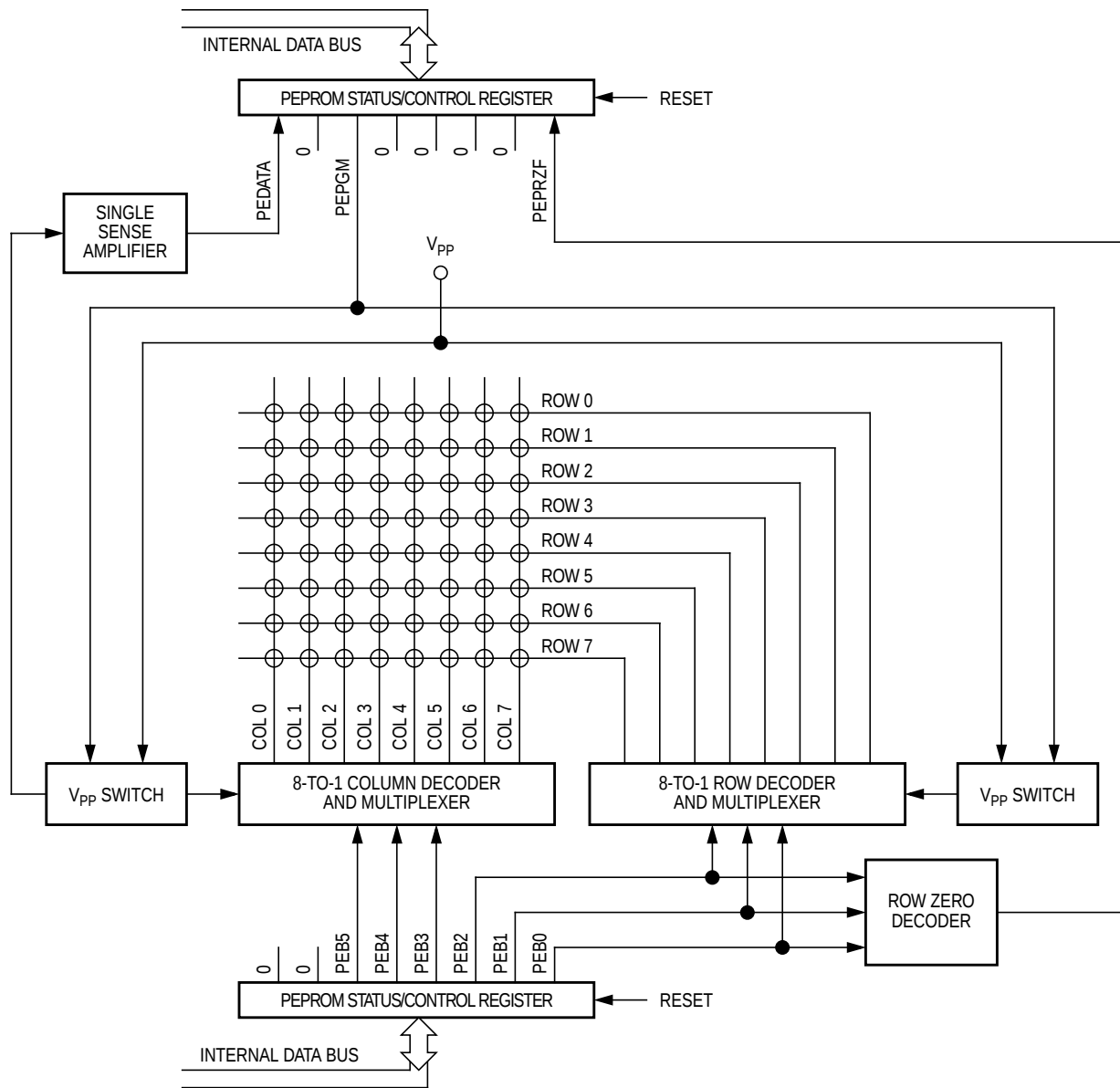
Figure 10-1. Personality EPROM
