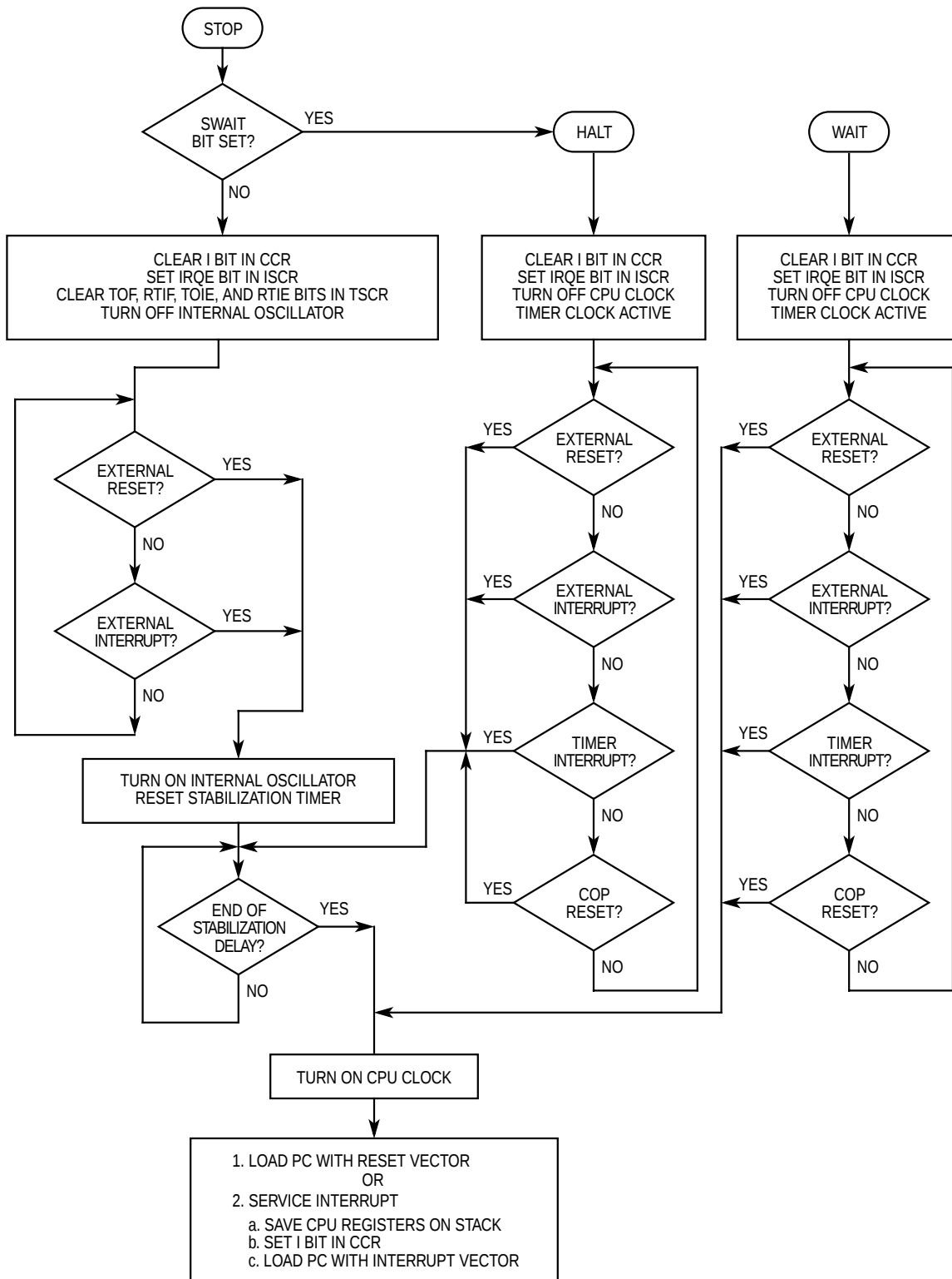
Figure 6-1. Stop/Wait/Halt Flowchart
