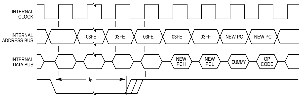
Figure 12-9. Power-On Reset Timing
