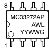
PDIP-8 P SUFFIX CASE 626
