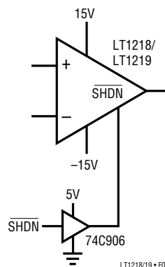
Figure 5. Shutdown Interface
