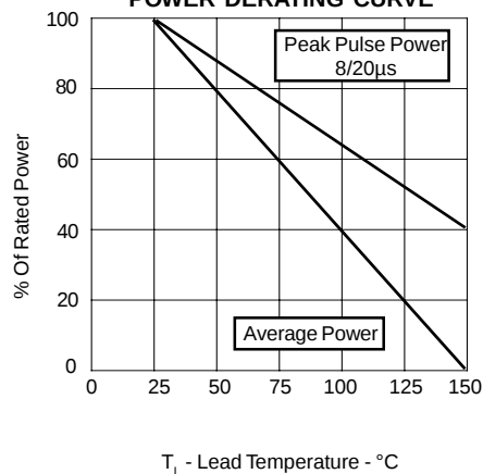
FIGURE 3 POWER DERATING CURVE
