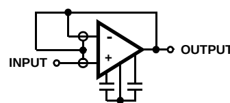
FIGURE 1B. FOLLOWER
