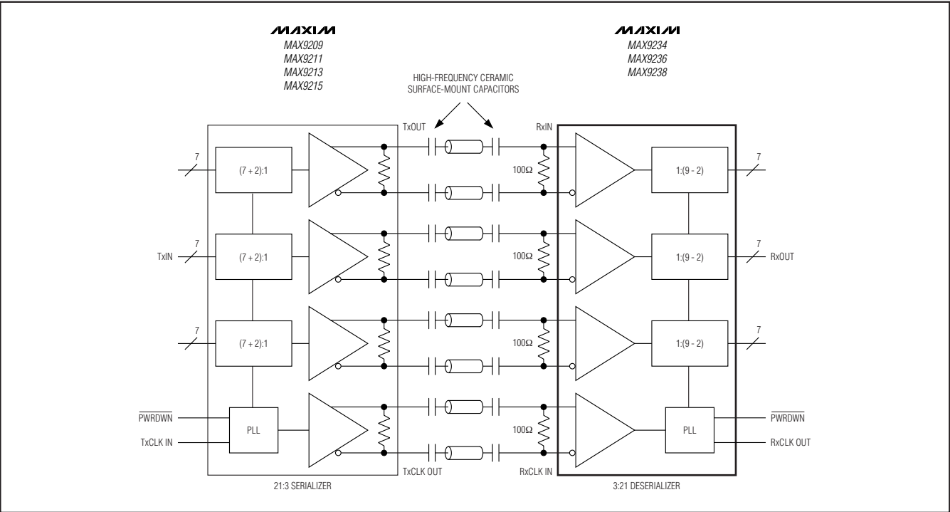
Figure 11. Four Capacitors per Link, AC-Coupled
