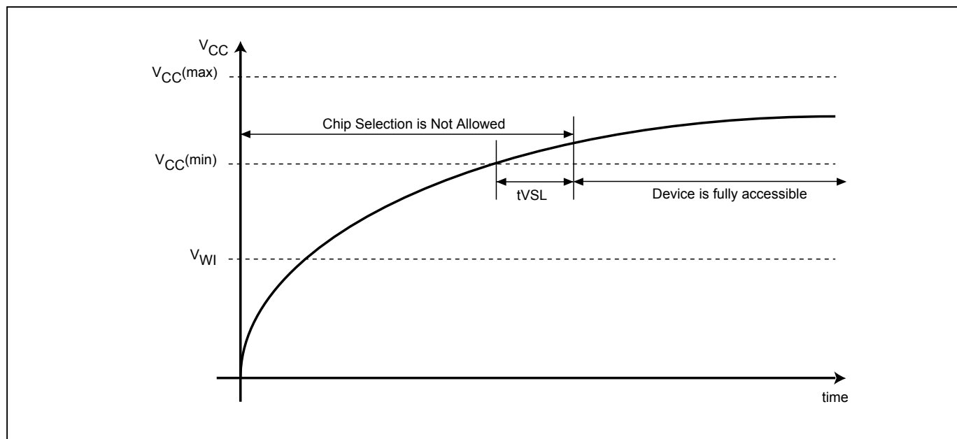
Figure 46. Power-up Timing
