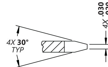
Section J-J
