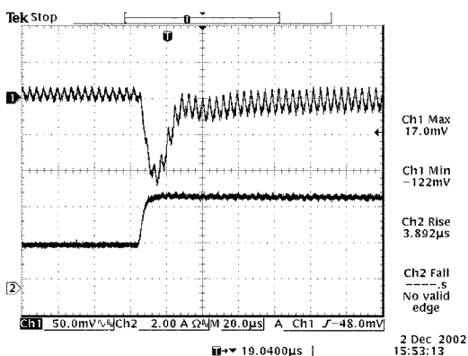
Vout=1.8V 50% to 100% load transients at 12V input and Ta=25° C
