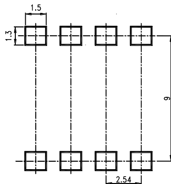
8 PIN
