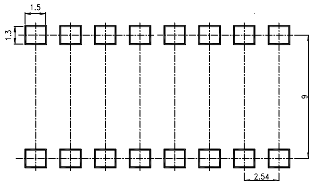
16 PIN
