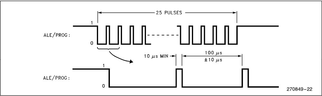
Figure 12. \overline{\text{PROG}} Waveforms
