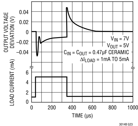
Transient Response
