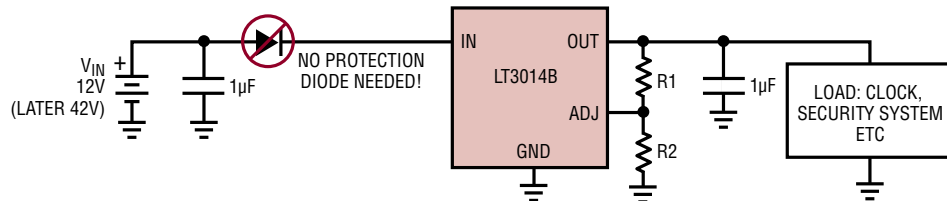
LT3014B Automotive Application
