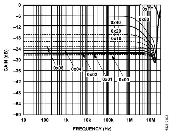
Figure 13. AD5252 Gain vs. Frequency vs. Code, R_{AB} = 1k\Omega , T_A = 25^\circ C
