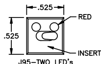
J95—TWO LED's
