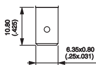
Quick-connect
