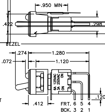
J95—TWO LED's
