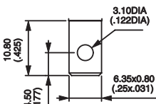
Sold.lug/Quick-conn.
