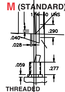
M (STANDARD) THREADED
