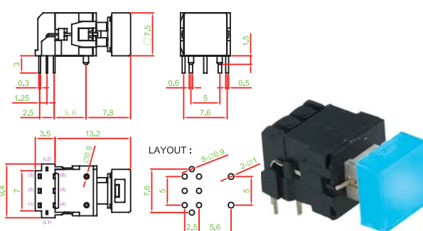
PS004-N22NR4S1XT□□□□
