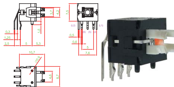
PS004-N22NRXXX□□□□
