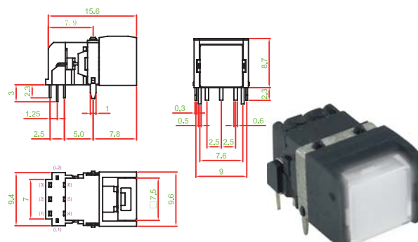
PS004-N22NR2S1KT□□□□
