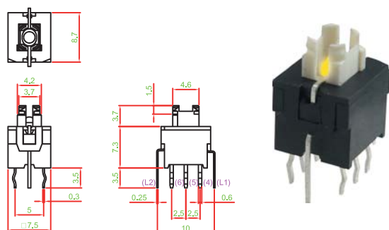
PS004-L22NPXXX□□□□
