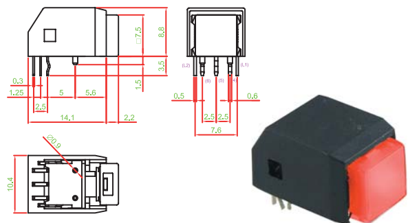
PS004-N22NR3S1KT□□□□
