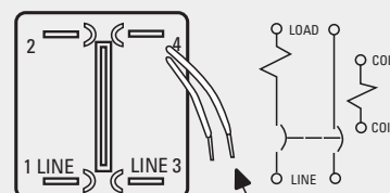
Two Pole (1 pole relay)
