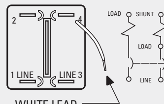
Two Pole (1 pole shunt)
