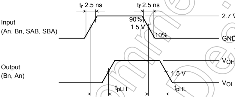
Figure 2 t_{pLH} , t_{pHL}
