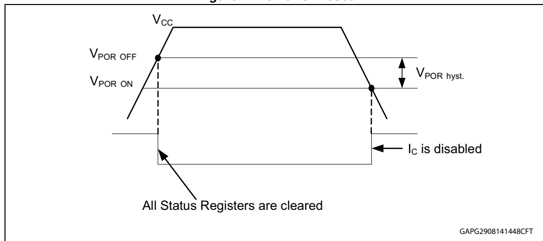
Figure 4. Power-on reset
