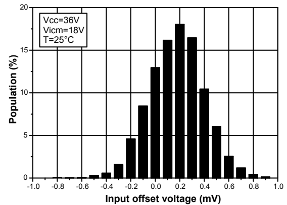
Figure 5. Input offset voltage distribution at V_{CC} = 36\text{ V}
