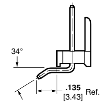
Retentive Leg
