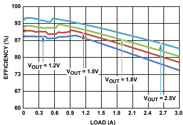
FIGURE 6. EFFICIENCY vs LOAD (ISL80031) f_{SW} = 1\text{MHz} , V_{IN} = 3.3\text{V} , PFM, T_A = +25^\circ\text{C}
