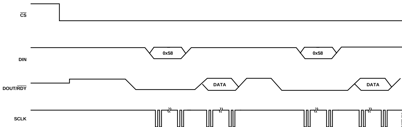
Figure 18. Continuous Conversion
