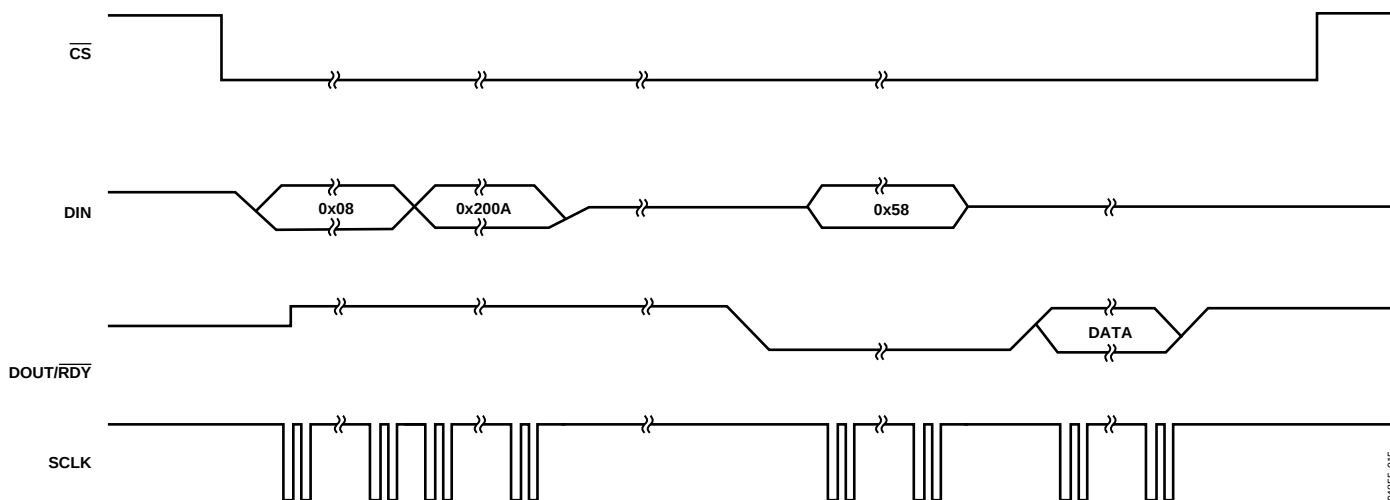
Figure 17. Single Conversion
