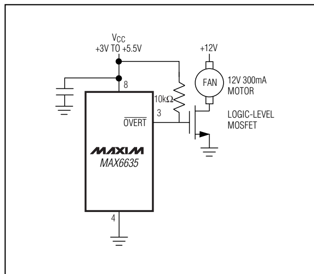
Figure 11. Fan Controller
