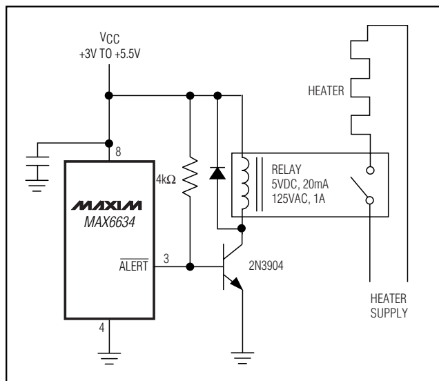
Figure 10. Simple Thermostat
