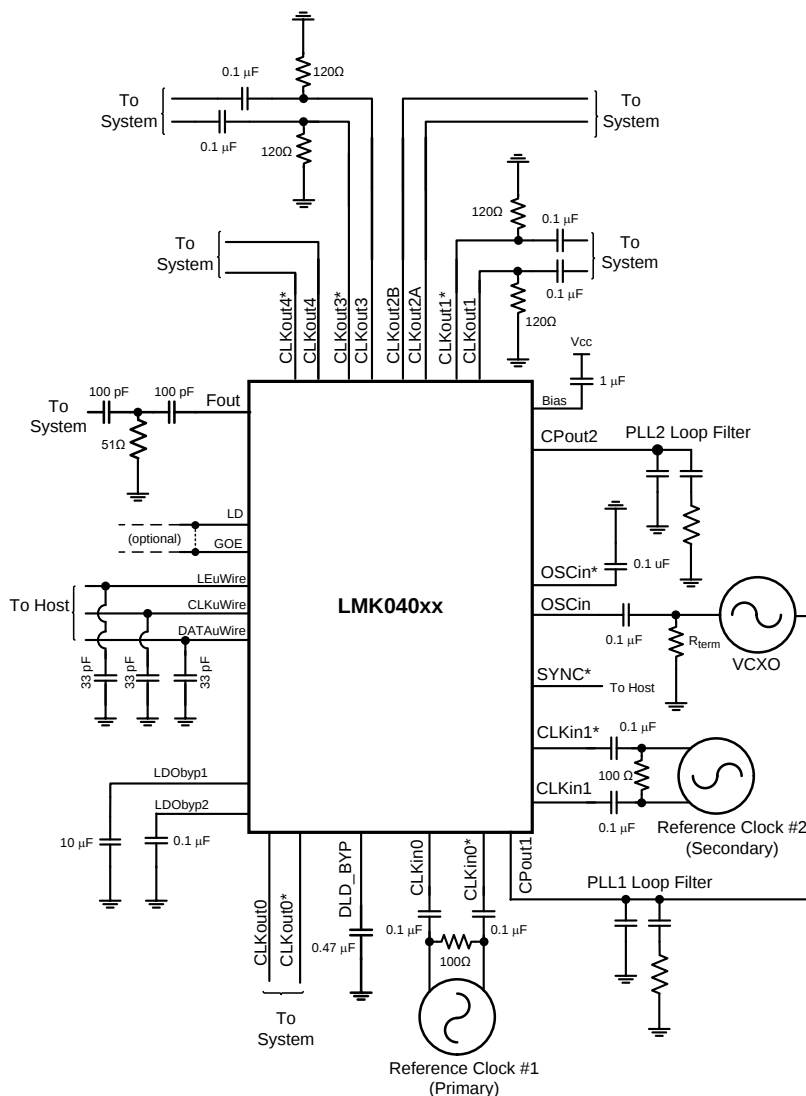
Figure 13. Typical Application
