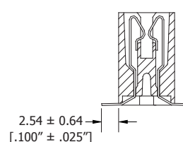
SURFACE MOUNT (HF)
