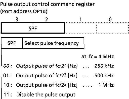
Figure 3-26. Pulse Output Command Register
