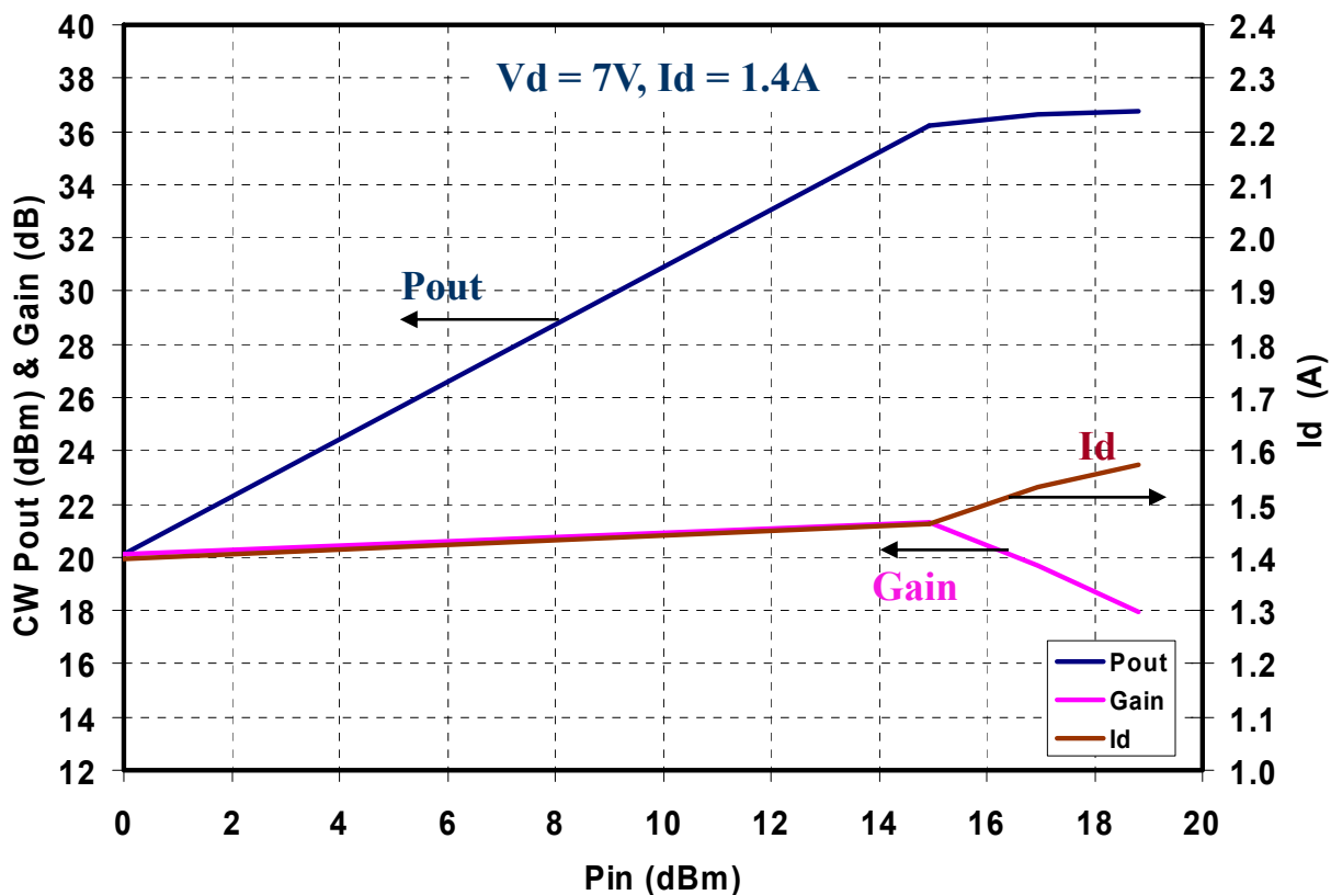
Measured Data Frequency @ 11GHz, CW Power
