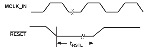
Figure 2. RESET Timing
