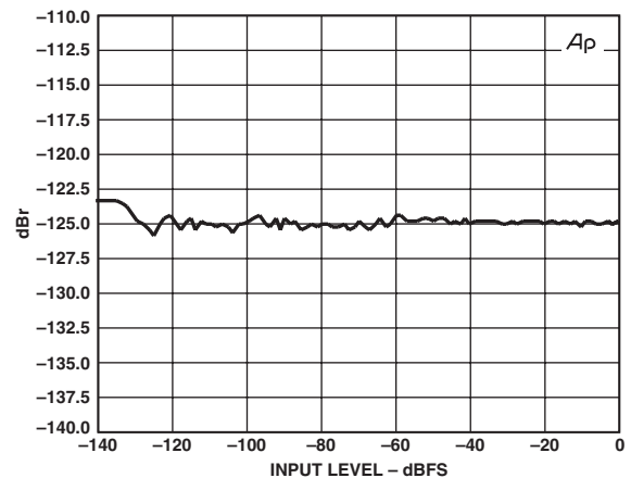
TPC 48. THD + N vs. Input Amplitude, 192 kHz: 48 kHz, 1 kHz Tone
