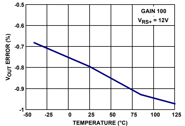
FIGURE 20. V_{OUT} ERROR (%) vs TEMPERATURE
