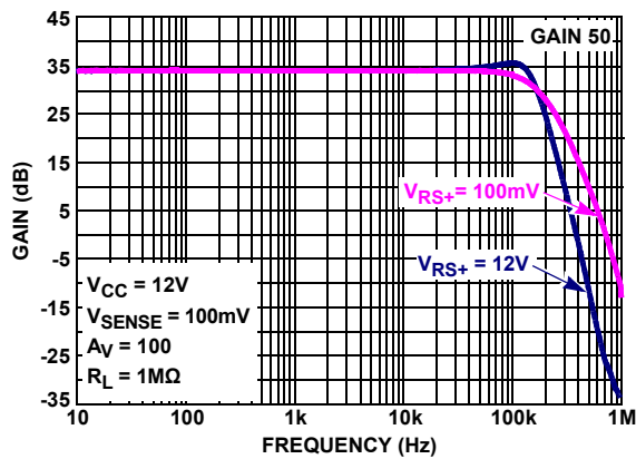
FIGURE 31. GAIN vs FREQUENCY V_{RS+} = 100mV/12V , V_{SENSE} = 100mV , V_{OUT} = 50mV_{p-p}
