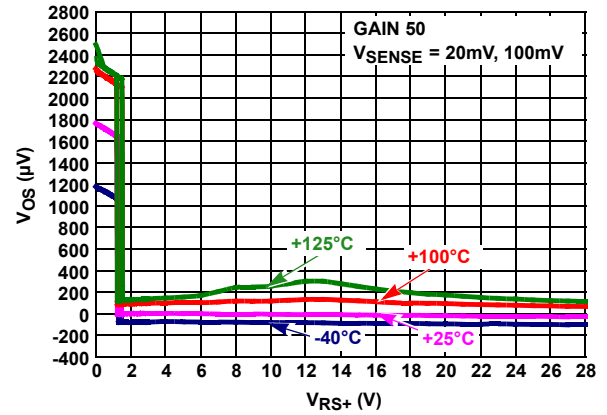
FIGURE 22. V_{OS} vs V_{RS+}
