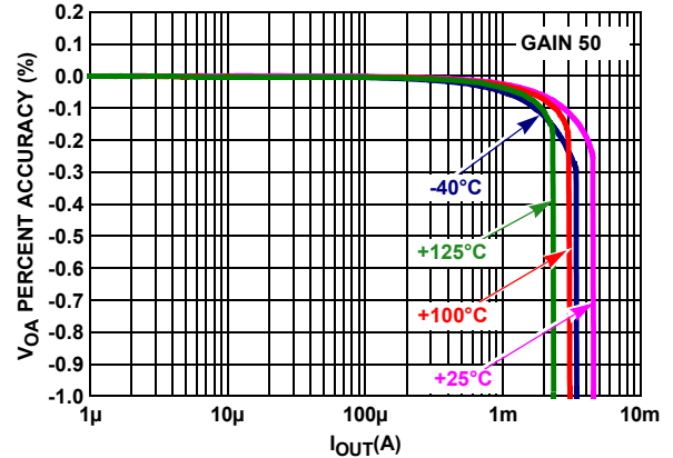
FIGURE 30. NORMALIZED V_{OA} vs I_{OUT}
