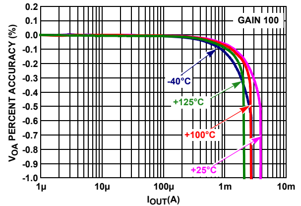
FIGURE 16. NORMALIZED V_{OA} vs I_{OUT}
