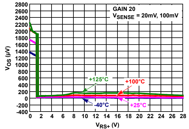
FIGURE 36. V_{OS} vs V_{RS+}
