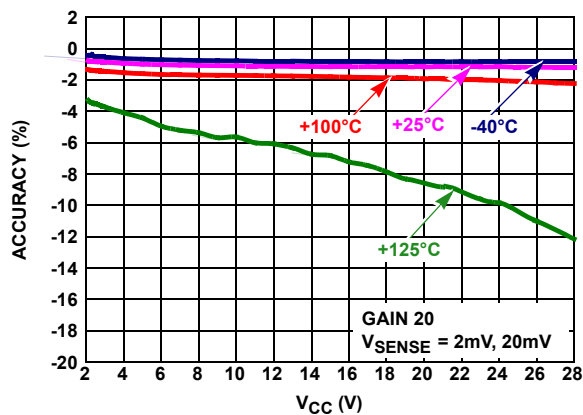
FIGURE 43. GAIN ACCURACY vs V_{CC} , LOW-SIDE
