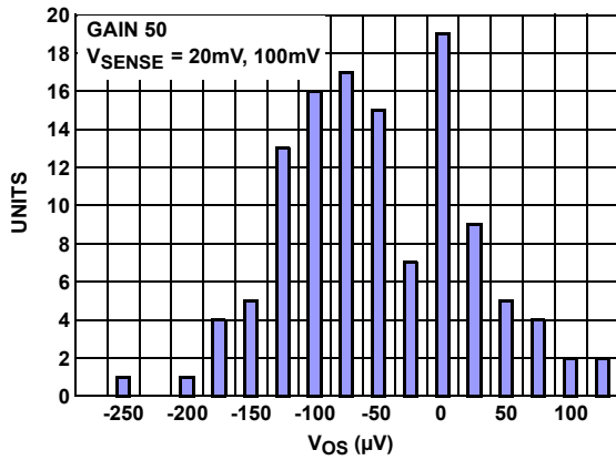
FIGURE 21. V_{OS} (μV) DISTRIBUTION AT +25°C, V_{RS+} = 12V , QUANTITY: 100
