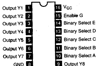
NTE74185 16-Lead DIP, See Diag. 249 Binary-to-BCD Code Converter
