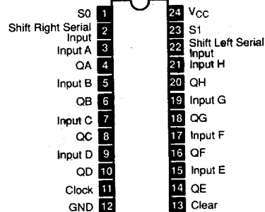
NTE74198 24-Lead DIP, See Diag. 252 8-Bit Bidirectional Universal Shift Register
