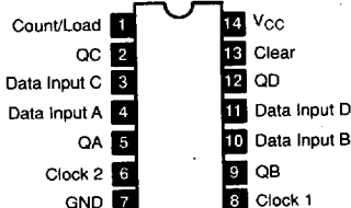
NTE74196, NTE74LS196, NTE74197, NTE74LS197 14-Lead DIP, See Diag. 247 Presetable Counter/Latch
