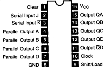
NTE74195, NTE74LS195A 16-Lead DIP, See Diag. 249 4-Bit Parallel Access Shift Register
