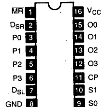
NTE74LS194, NTE74LS194A, NTE74S194 16-Lead DIP, See Diag. 249 4-Bit Bidirectional Universal Shift Register
