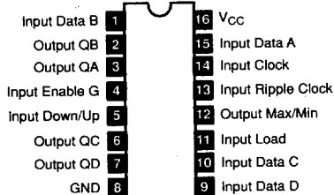
NTE74LS190, NTE74191, NTE74LS191 16-Lead DIP, See Diag. 249 Synchronous Up/Down Counter
