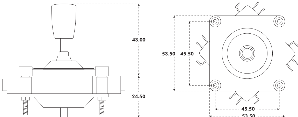
V3 SCREW MOUNT
