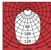
Polar Diagram Micro-Lynx F
