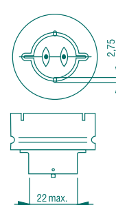
BY 22d
