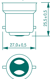
B22d/BC
