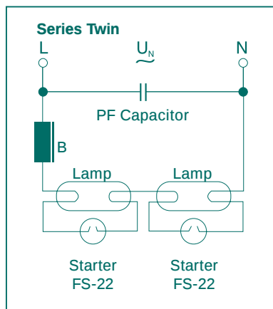
Series Twin with conventional ballast only with 2 x FS-22 starter Lynx-L 18W
