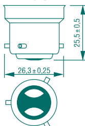
B22d-3
