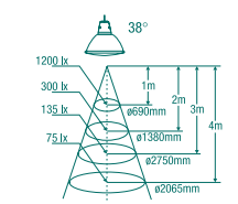
Coolfit 50W / 38°
