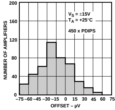
Figure 1. OP193 Offset Distribution, V_S = \pm 15\text{ V}
