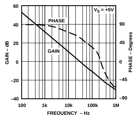
Figure 21. Open Loop, Gain and Phase vs. Frequency
