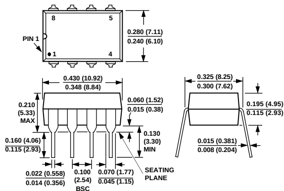
8-Lead Epoxy DIP (P Suffix)
