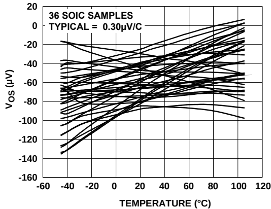
FIGURE 19. EL8176SOIC V_{OS} vs TEMPERATURE ( V_S = 5V )
