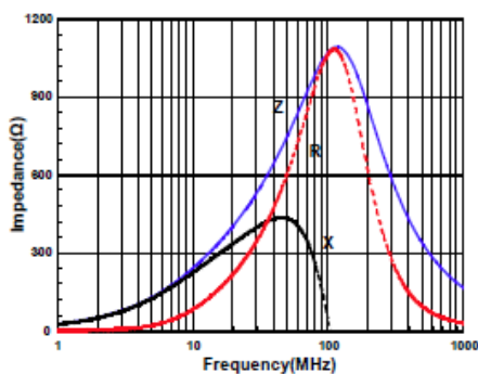
ACML-0402H-102
