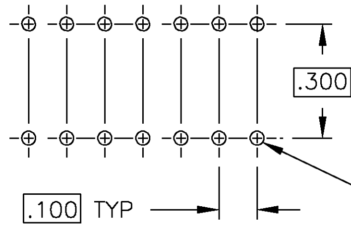
RECOMMENDED MOUNTING HOLE PATTERN SCALE 4:1
