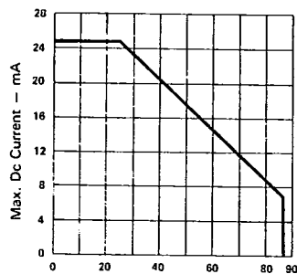
5-161 Fig. 4 MAX. ALLOWABLE DC CURRENT PER SEG. Vs AMBIENT TEMPERATURE.
