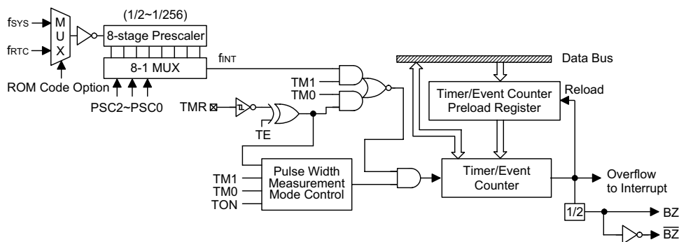
Timer/Event Counter
