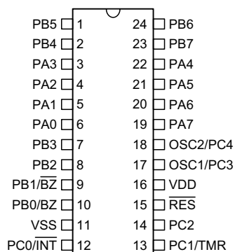
HT48R10A-1 - 24 SKDIP-A/SOP-A
