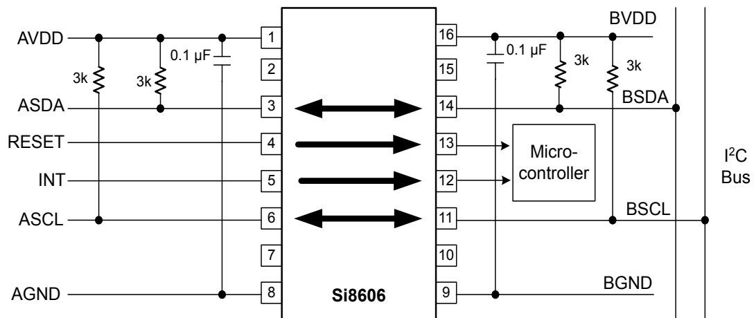
Figure 3.7. Typical Si8606 Application Diagram
