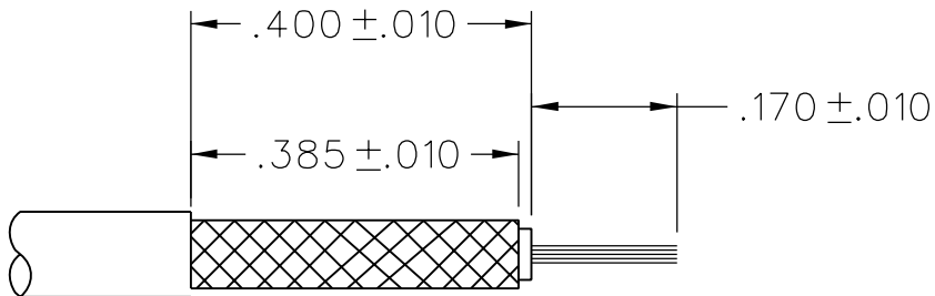
CABLE STRIP DIMENSIONS NOT TO SCALE
