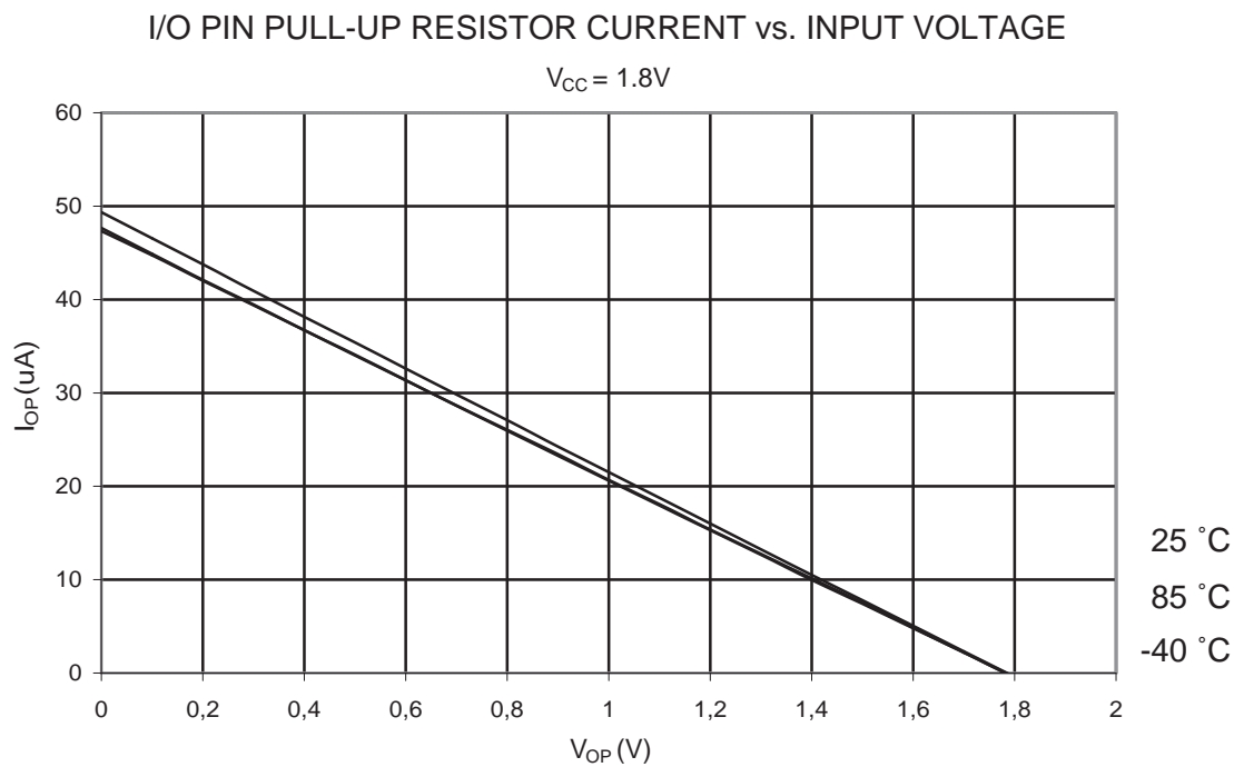
Figure 20-20. Pull-Up Resistor Current vs. Input Voltage (I/O Pin, V_{CC} = 1.8V )
