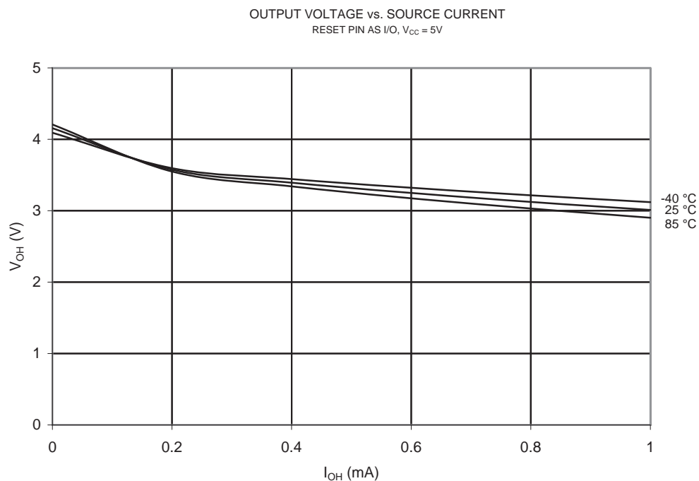
Figure 20-85. V_{OH} : Output Voltage vs. Source Current (Reset Pin as I/O, V_{CC} = 5\text{V} )
