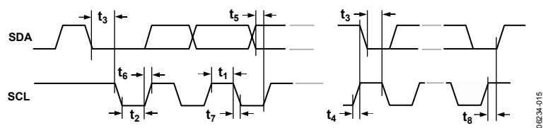
Figure 15. MPU Port Timing Diagram (I²C Mode)
