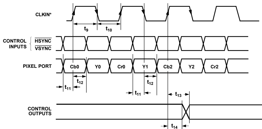
Figure 6. ED/HD-DDR Input, 8-/10-Bit 4:2:2 YCrCb (HSYNC, VSYNC), Input Mode 010
