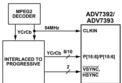
Figure 60. ED (At 54 MHz) Example Application
