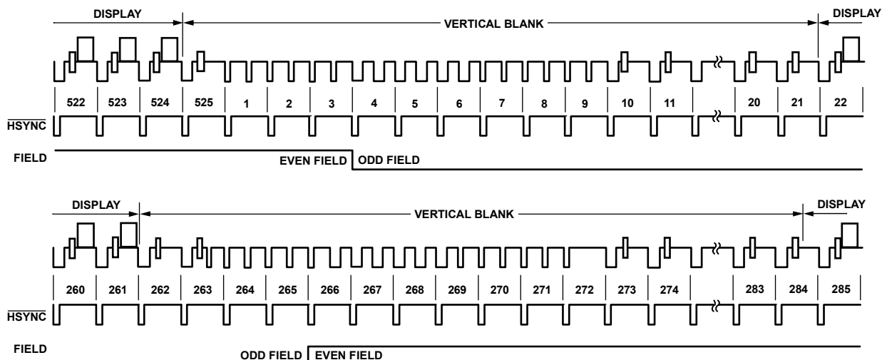
Figure 106. SD Timing Mode 1, Slave Option, NTSC
