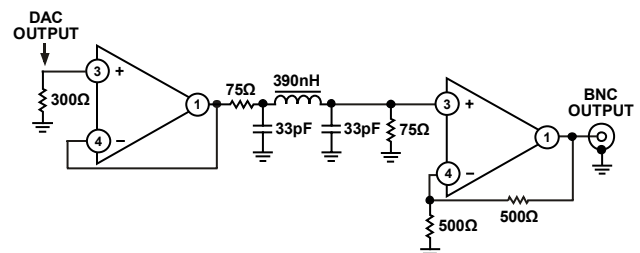
Figure 88. Example of Output Filter for HD, 4 \times Oversampling
