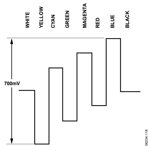
Figure 118. Pb Levels—NTSC
