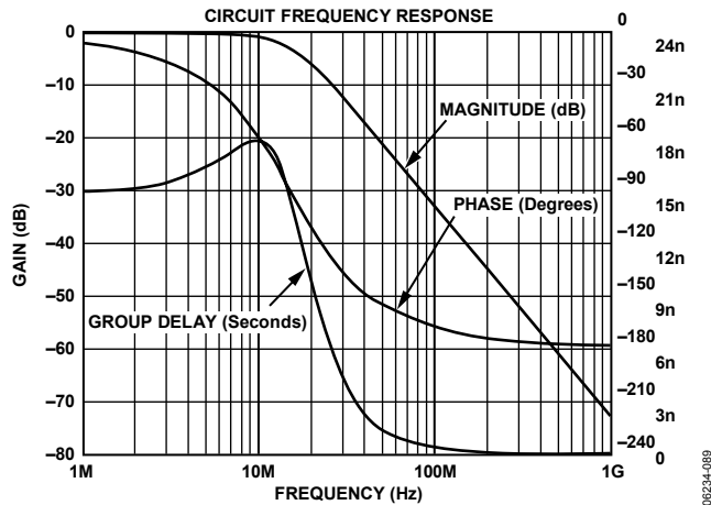
Figure 89. Output Filter Plot for SD, 16x Oversampling
