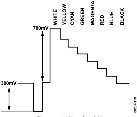
Figure 119. Y Levels—PAL
