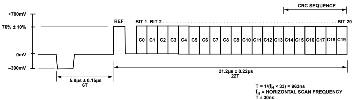
Figure 94. Enhanced Definition (525p) CGMS Waveform
