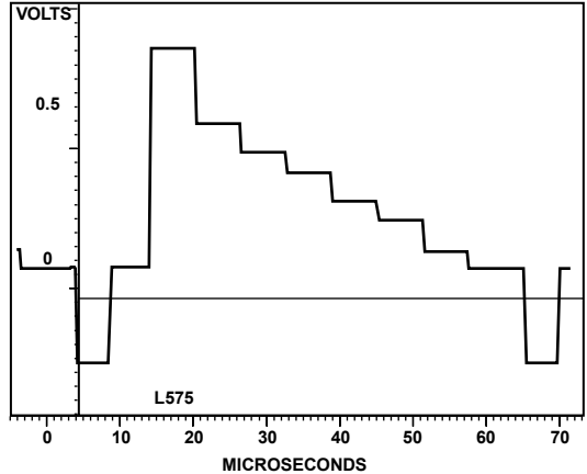
Figure 134. PAL Luma
