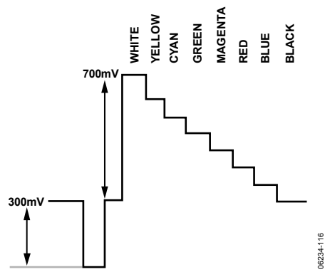
Figure 116. Y Levels—NTSC
