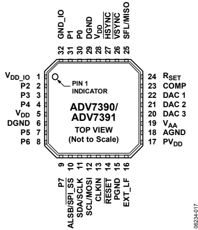
Figure 17. ADV7390/ADV7391 Pin Configuration
