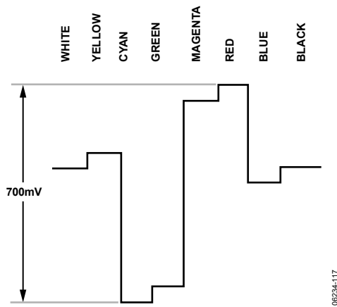
Figure 117. Pr Levels—NTSC
