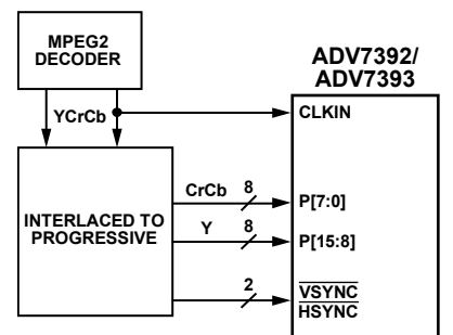
Figure 57. ED/HD-SDR Example Application
