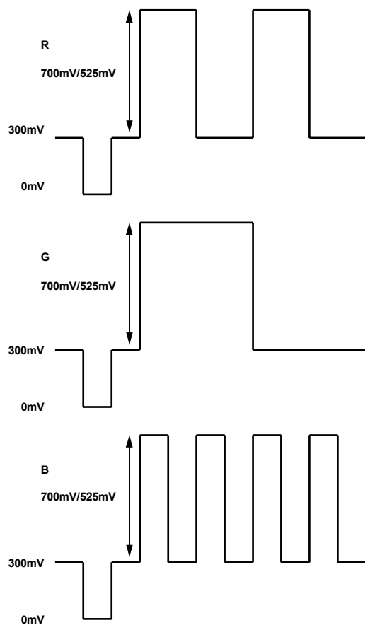
Figure 127. SD/ED RGB Output Levels—RGB Sync Enabled
