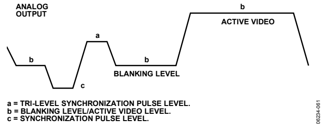
Figure 61. ED/HD Nonstandard Timing Mode Output Levels
