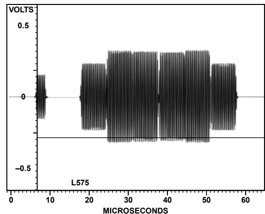
Figure 135. PAL Chroma
