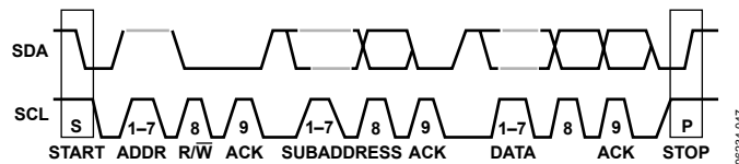
Figure 47. I²C Data Transfer
