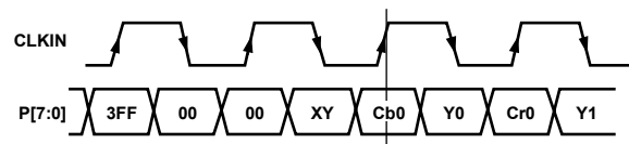
Figure 50. ED/HD-DDR Input Sequence (EAV/SAV)—Option A
