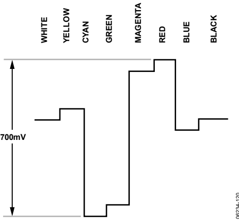
Figure 120. Pr Levels—PAL
